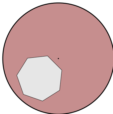
Figure 165: An edge case of the circle/polygon check
